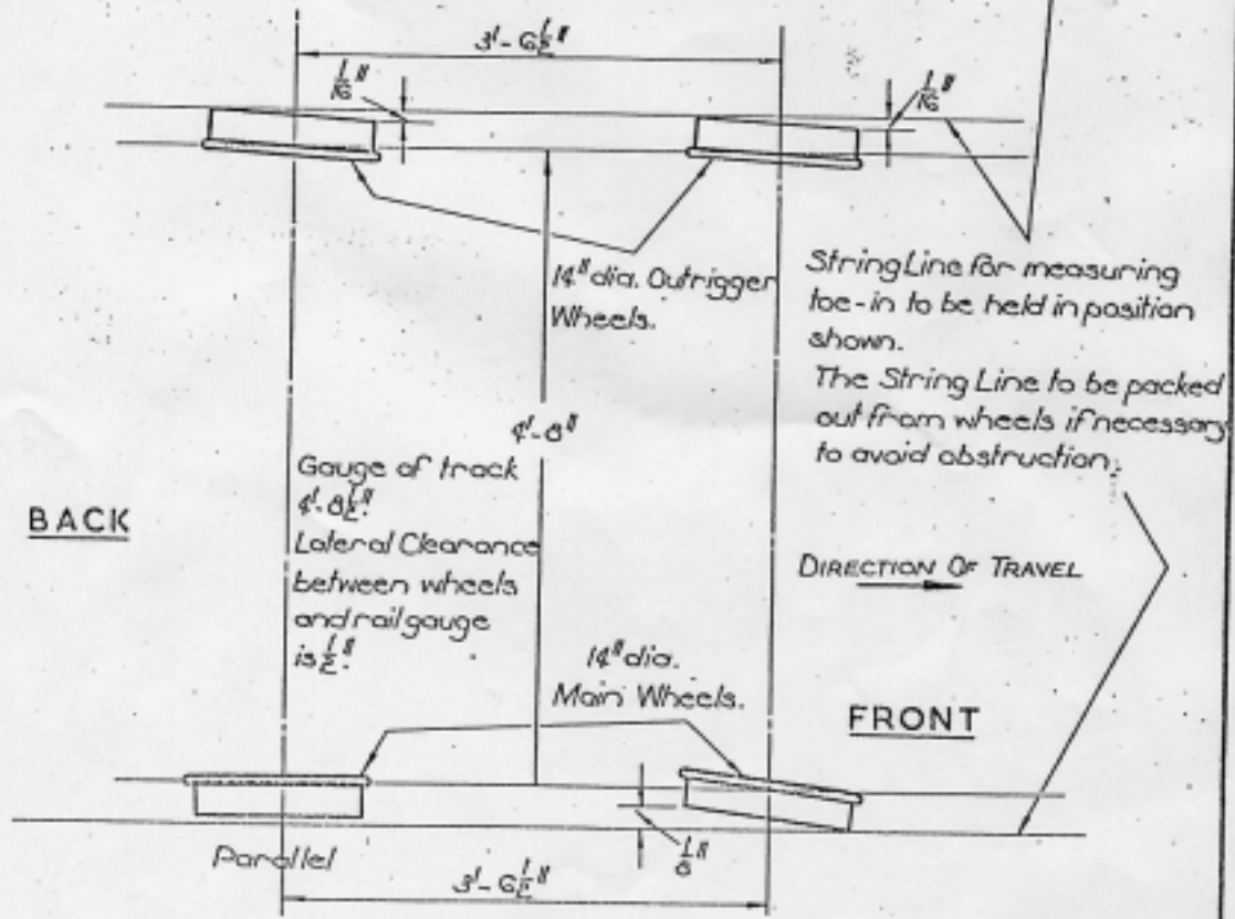
PLAN OF WHEELS
